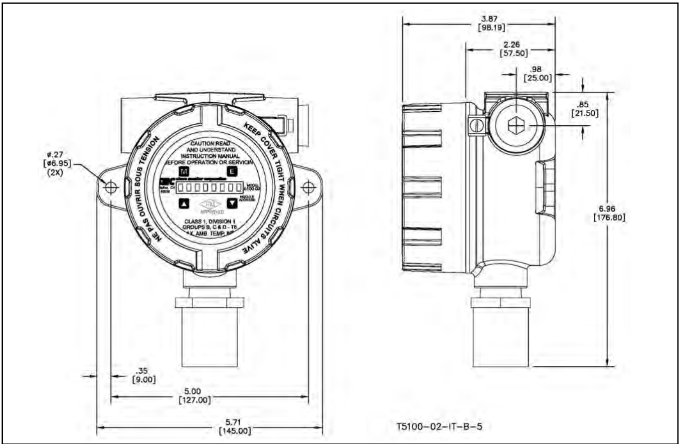
Figure 1 - 3: Model 5100-02-IT-A1 (and A2) Combustible Sensor – Cast Aluminum Enclosures, Dimensions
