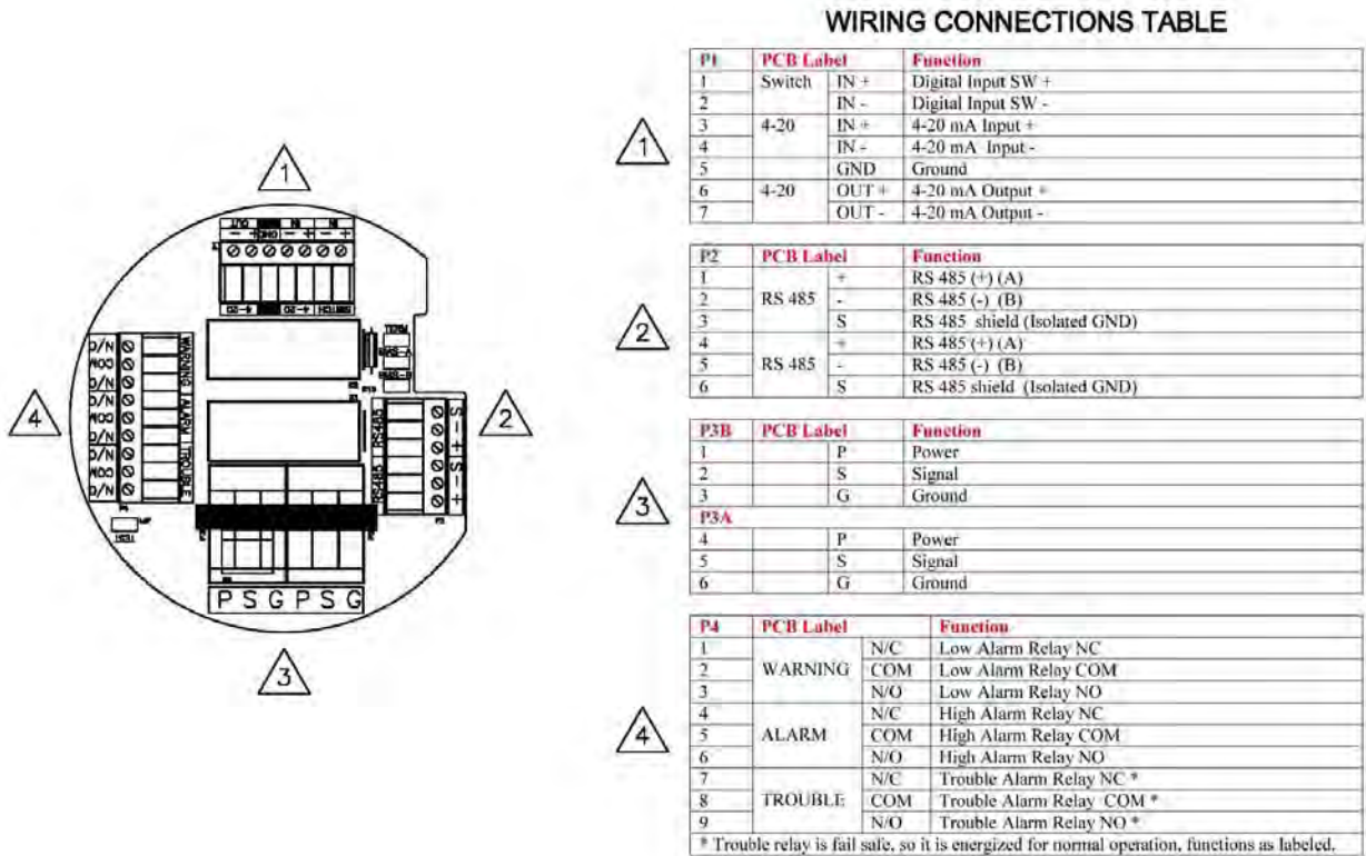
Figure 4 - 7: Termination Drawing
